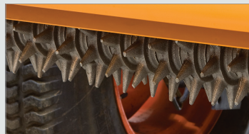
Studded roller for minimal surface disturbance and creating the seedbed ‘plant pots’
