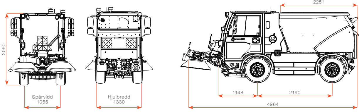
Citymaster 2250 – 2-borstversion
