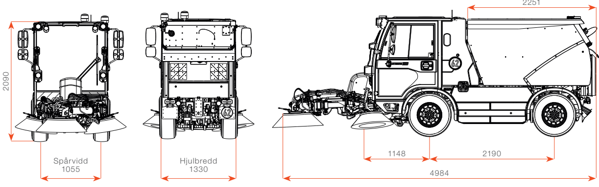
Citymaster 2250 – 3-borstversion
